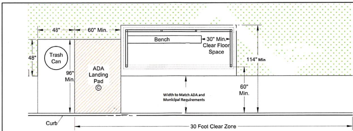
Figure 22: Bus Shelter with Adjacent Sidewalk and ADA Landing Pad Next to Shelter. Source: COTA Bus Stop Guidelines
