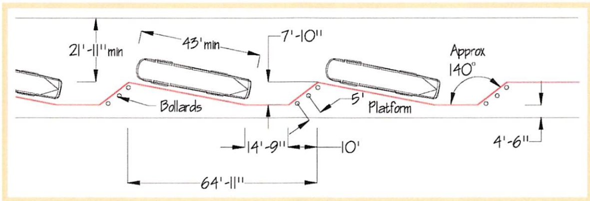
Figure 9: Example of Sawtooth Bus Bay
