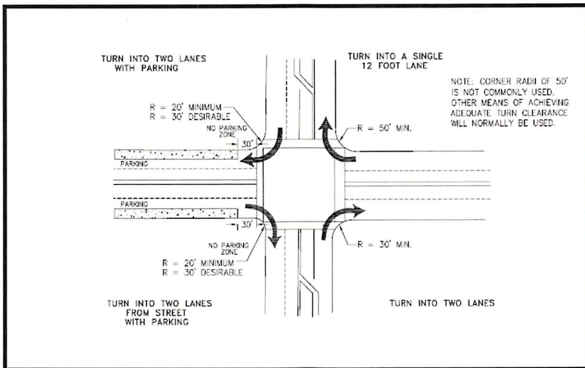
Figure 32: Represents Curb Design for Bus Turning. Source: Darnell and Associates INC.
