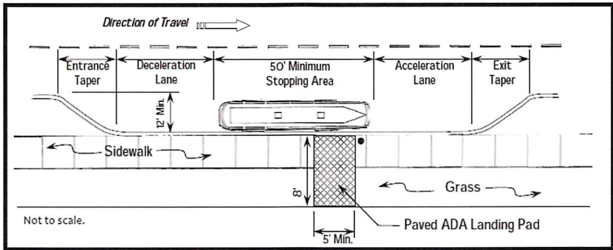
Figure 8: Example of Parallel Bus Bay
