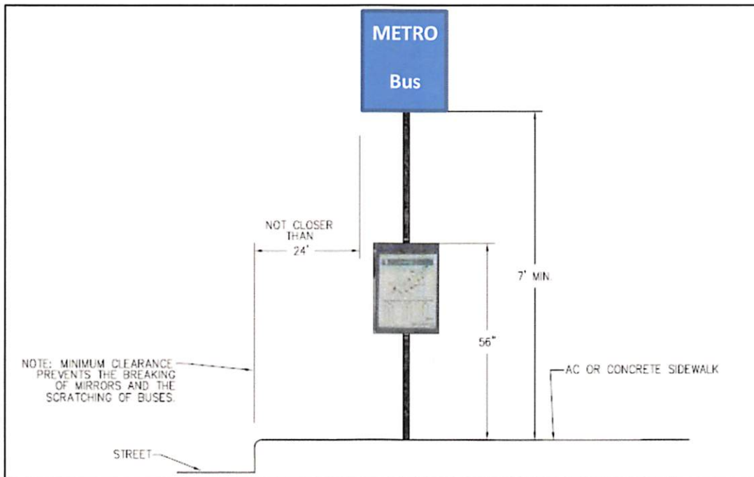
Figure 15: Bus Stop Sign Placement Criteria Source: Damell and Associates INC.
