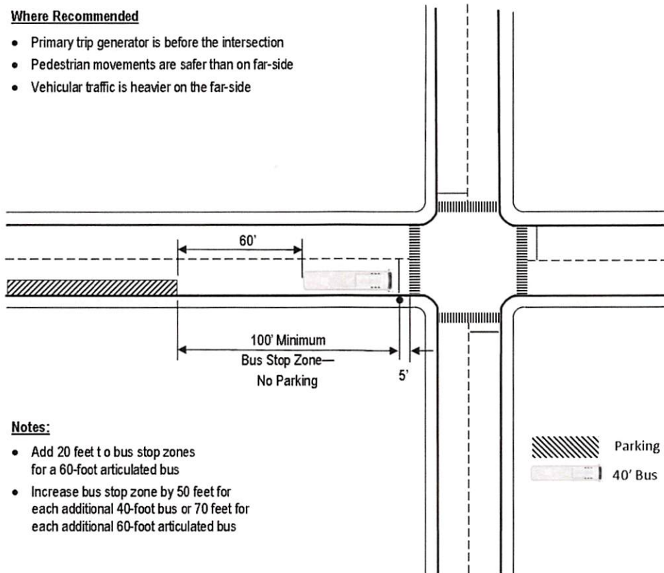
Figure 2: Example of Near-Side Bus Stop
