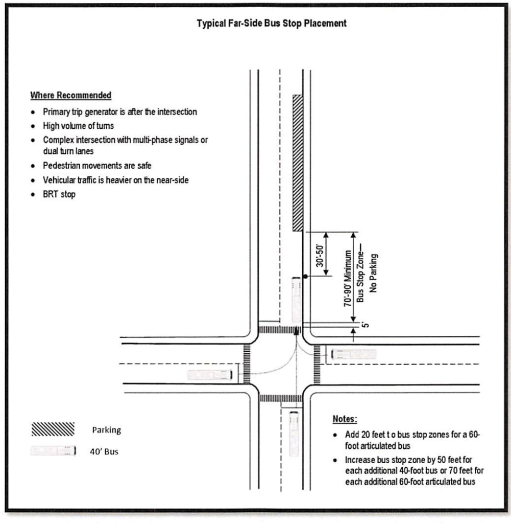
Figure 1: Example of Far-Side Bus Stop
