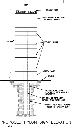
PROPOSED PYLON SIGN ELEVATION N.T.S.
